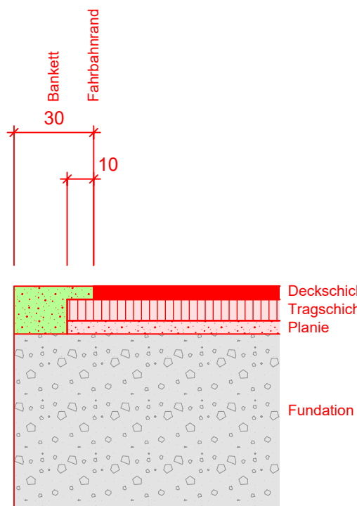
Detail Belagsrand, 1:20
