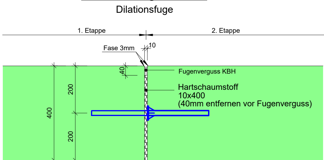
Detail Fuge, 1:10
